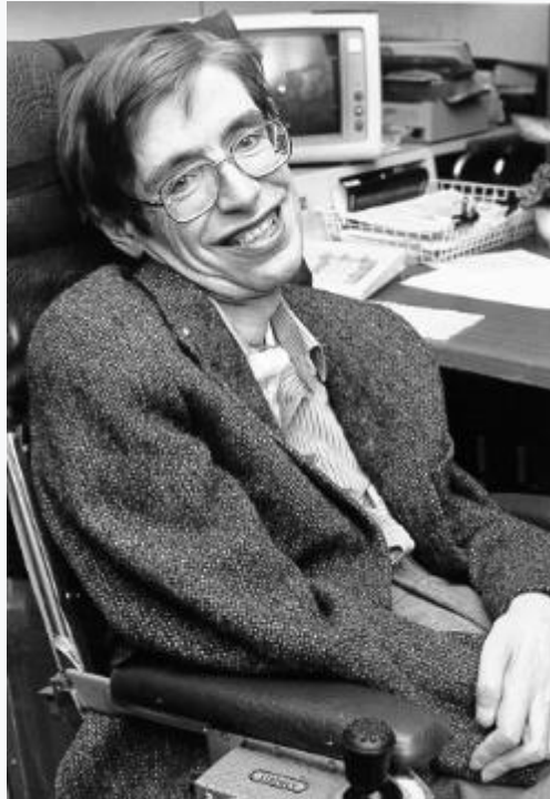
Hawking, c. 1980
